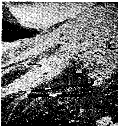
Figure 9. Typical horizontal drain installations.
